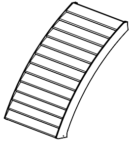
Item 12 Left Side Roof Panel X 1
